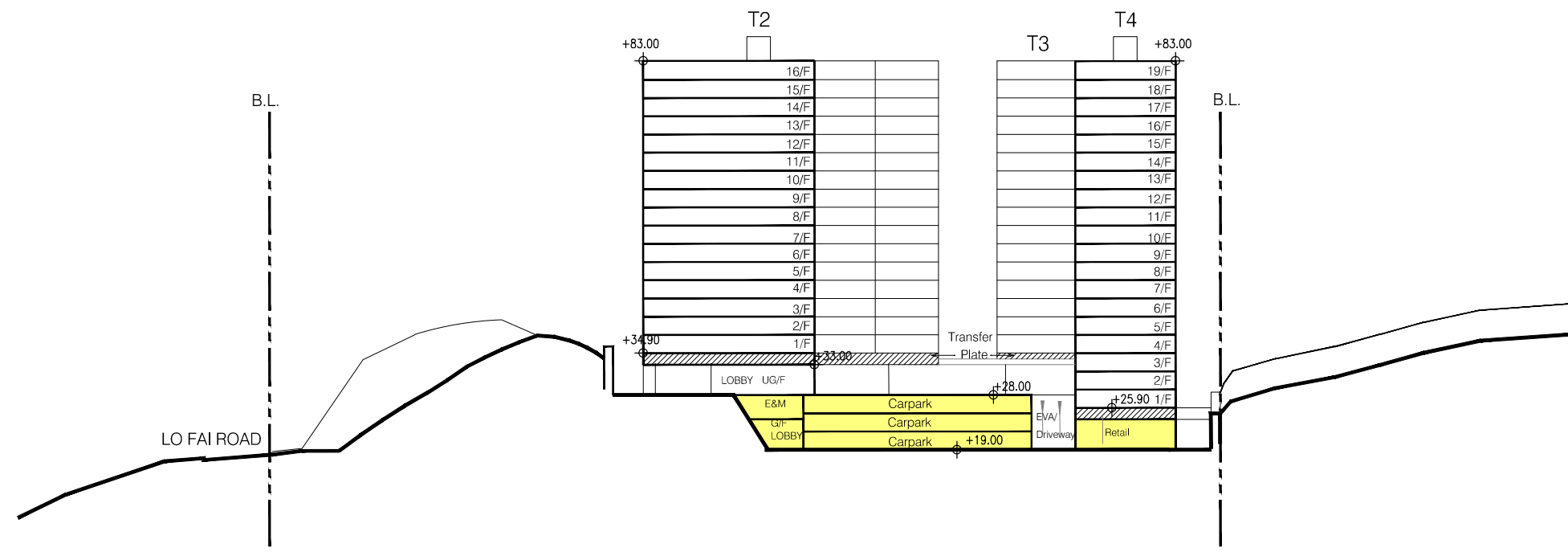
Section C-C
